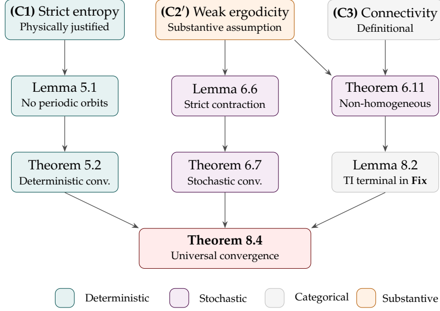
Figure 1: Proof dependency diagram. The three conditions (top row) feed into intermediate lemmas (middle) and the main theorems (bottom), culminating in Theorem 8.4. Colour encodes the proof track: teal for deterministic, purple for stochastic, grey for categorical, and amber for the single substantive physical assumption (C2').
